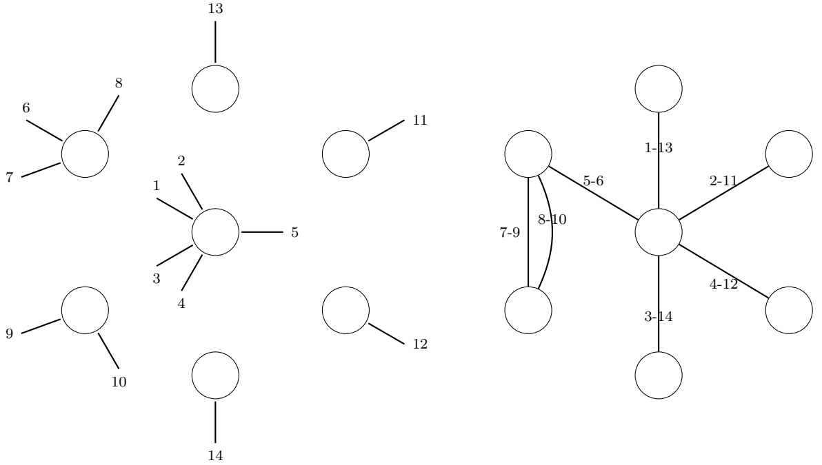
(a) Stubs generated from a scale-free degree sequence (b) Stubs paired uniformly at random into edges
